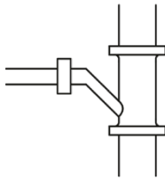
3-way connection of the condensate pipe Connection of a drain elbow
