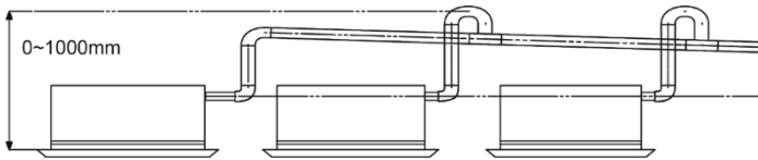
Condensate pipes converging towards a T-piece
